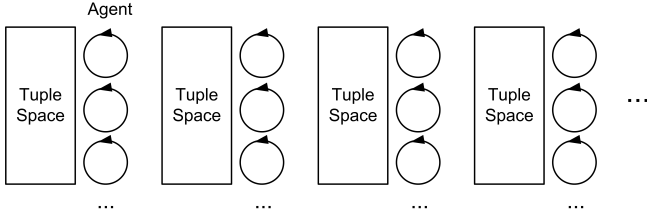
Fig. 1. The basic architecture consists in a set of sorter agents dedicated to a single tuple space.
